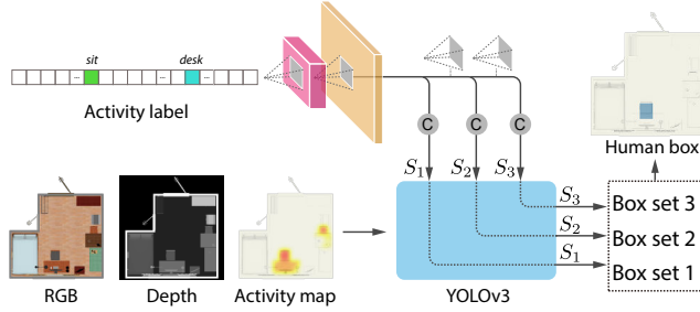
Fig. 4. Our activity localization network. The architecture is based on the YOLOv3 [Redmon and Farhadi 2018] approach and takes as input the RGBD representation of top-down view image of a room, an activity label and the corresponding predicted activity map, and predicts bounding boxes with corresponding human pose types.
