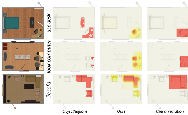
Fig. 10. Comparison of our method to the object-centric baseline.
