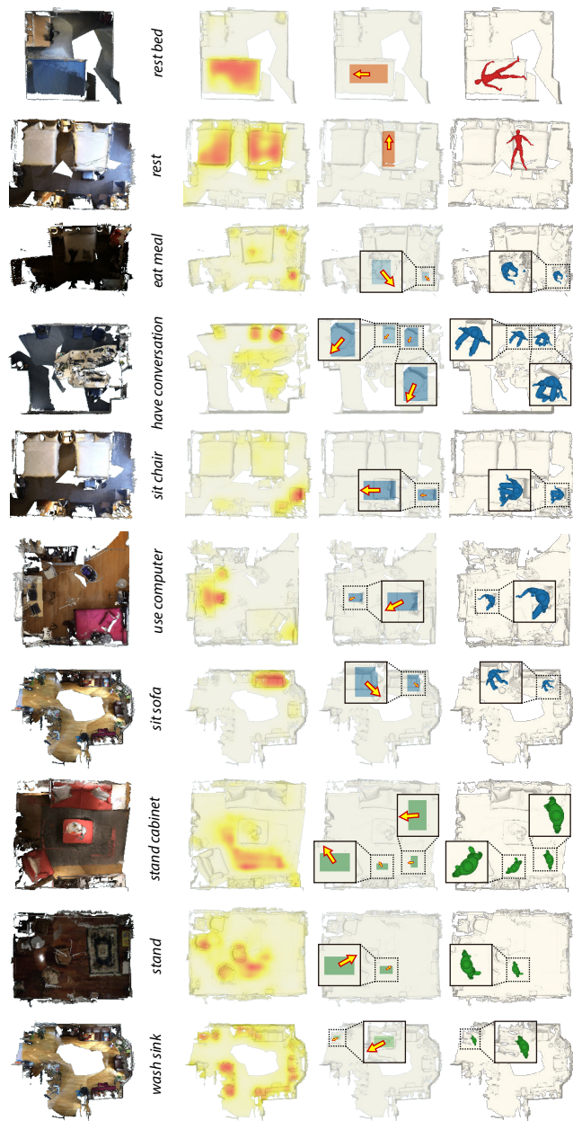
Fig. 14. Activity prediction and hallucination results on scans of real rooms from ScanNet [Dai et al. 2017]. See the supplementary material for additional 3D views.
