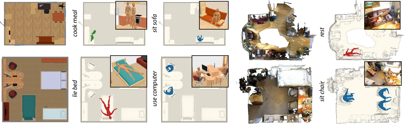
Fig. 1. We develop deep neural networks for functional understanding of 3D scenes, through human activity prediction and hallucination in both synthetic (left) and reconstructed (right) indoor environments. In each of the four examples, the leftmost image shows an input scene with no humans. Images to the right show predicted activities and their hallucination with associated human poses to illustrate the scene functionalities (top-down view with 3D view inset).
