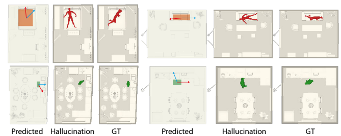
Fig. 13. Examples of activity hallucination results with large orientation error but still valid. We show two examples for lying poses (first row) and two examples for standing poses (second row). For each example, from left to right, we show the predicted human box with ground-truth orientation (blue arrow) and predicted orientation (red arrow), the scene with a hallucinated human in the predicted orientation, and the ground-truth pose orientation.
