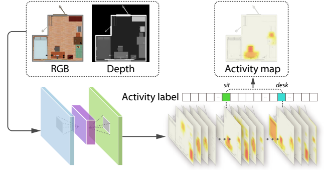
Fig. 3. Our activity prediction network. The network is an encoder-decoder which takes as input the top-down view image of a scene represented with RGB and depth channels and outputs a probability map for each of the \omega = 34 words in our dataset. Then, for each activity label, we take one word map (for verbs) or merge two word maps (for verb-noun tuples) to obtain the corresponding activity map.
