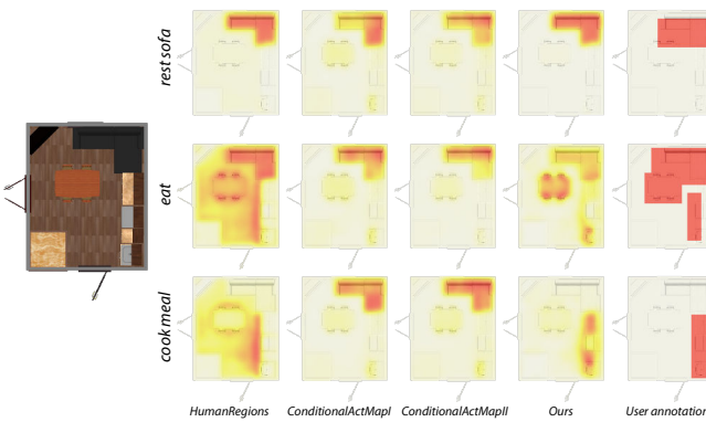
Fig. 11. Comparison of different activity prediction methods.
