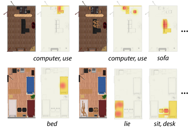
Fig. 9. Comparison of word maps obtained from input rooms with and without observed humans. Left: the only word map obtained for the given scene without human. Right: some examples of word maps obtained for the same scene but with a human present.
