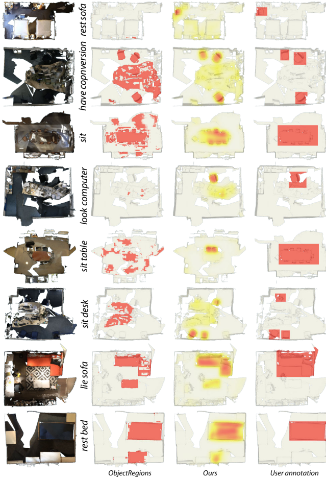
Fig. 15. Comparison of our method to the object-centric baseline on rooms from ScanNet [Dai et al. 2017]. Our method is more precise and produces results more similar to the ground-truth in many of the cases.
