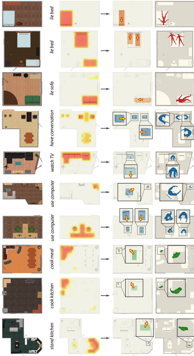
Fig. 8. Examples of human activity hallucination. From left to right, we show the input room, activity map corresponding to the input activity label, the detected human bounding boxes with predicted pose type and orientation, and the final hallucinated human poses in the input room. See the supplementary material for additional 3D views. The predicted poses are positioned and oriented realistically, demonstrating how people use objects during the input activity.
