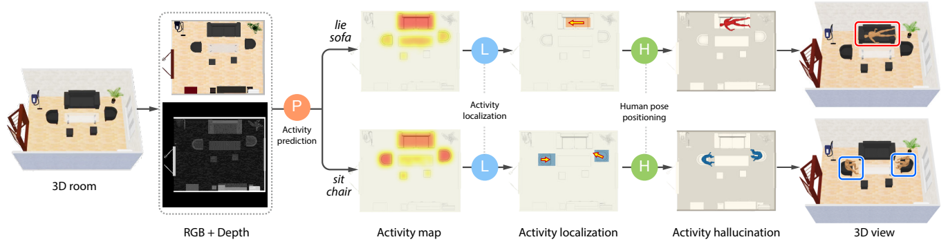
Fig. 2. Overview of our activity prediction and hallucination method: given an unlabeled indoor scene without human presence, represented by a top-down RGBD view, a deep network P predicts activity maps that indicate where and what different activities can be supported in the scene. Next, an activity localization network L predicts coarse parameters (i.e., human bounding boxes, types and orientations) which guide the positioning of human poses (labelled by H ) to illustrate human activities predicted by the action maps.
