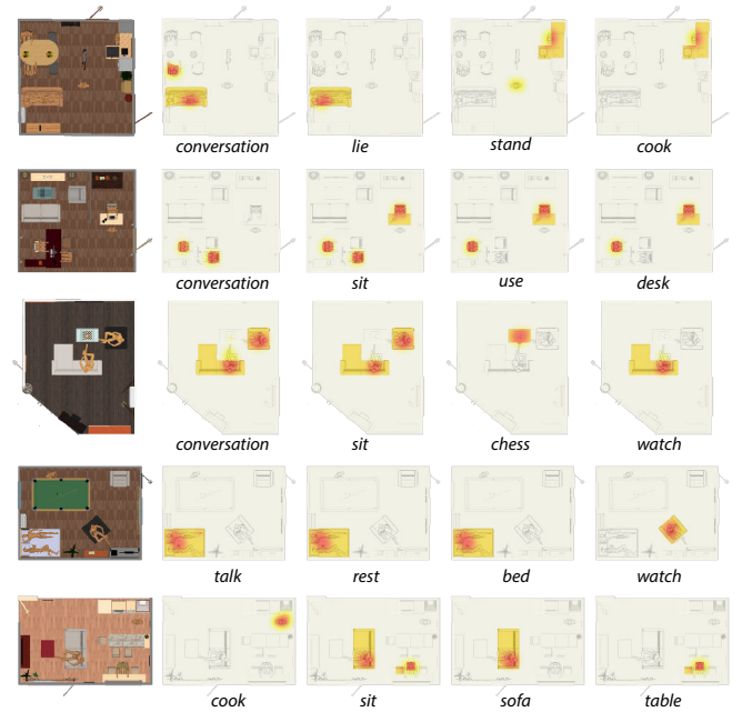
Fig. 6. Examples of training data for activity map prediction. For each input scene on the left, we show different word maps generated from our human activity annotated data. Note the natural emergence of correlations between related verbs and objects, such as cook and a kitchen counter, and subtle differences between maps corresponding to different but related words, e.g., conversation and lie or conversation and sit in the first two rows.
